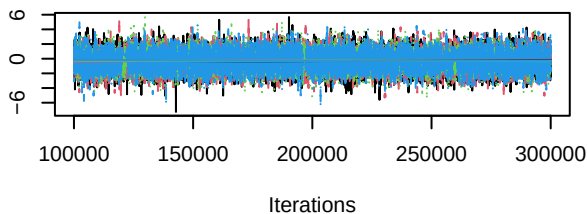
Trace of d.III.III_Amivantamab
