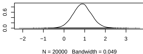
Density of d.III.III_antiangio
