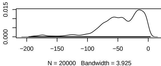
Density of d.III.III_PD_L1i
