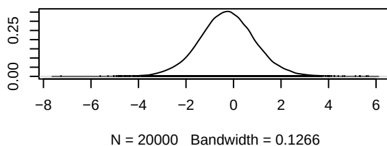
Density of d.III.III_Amivantamab
