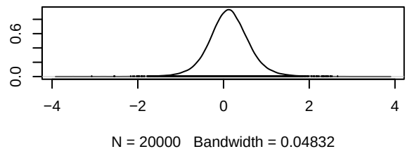
Density of d.I.Zorifertinib
